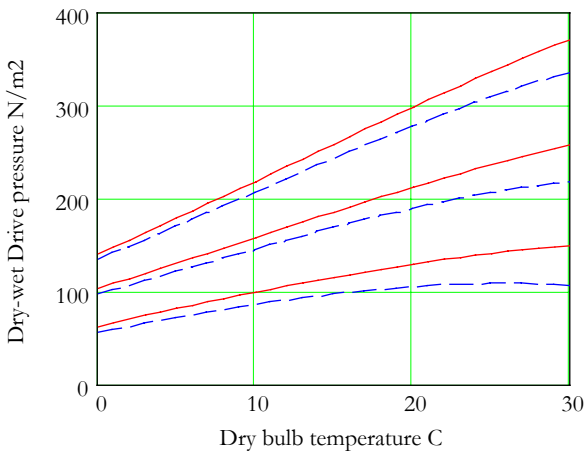
Figure 7. Driving pressure for evaporation at 60, 70, 80% RH.
